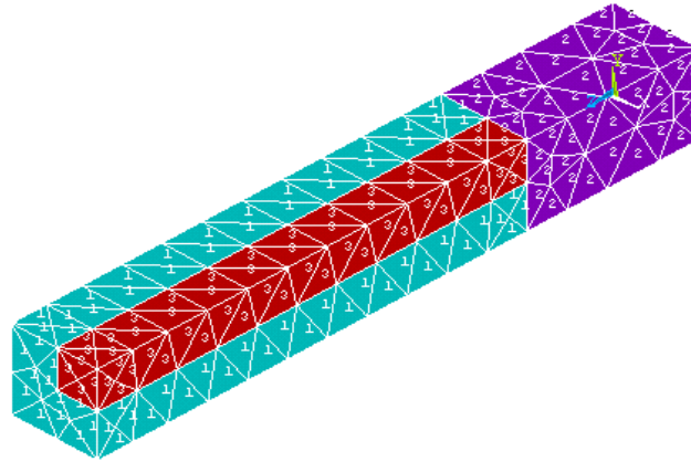
Fig.4 Three dimensional mesh.
