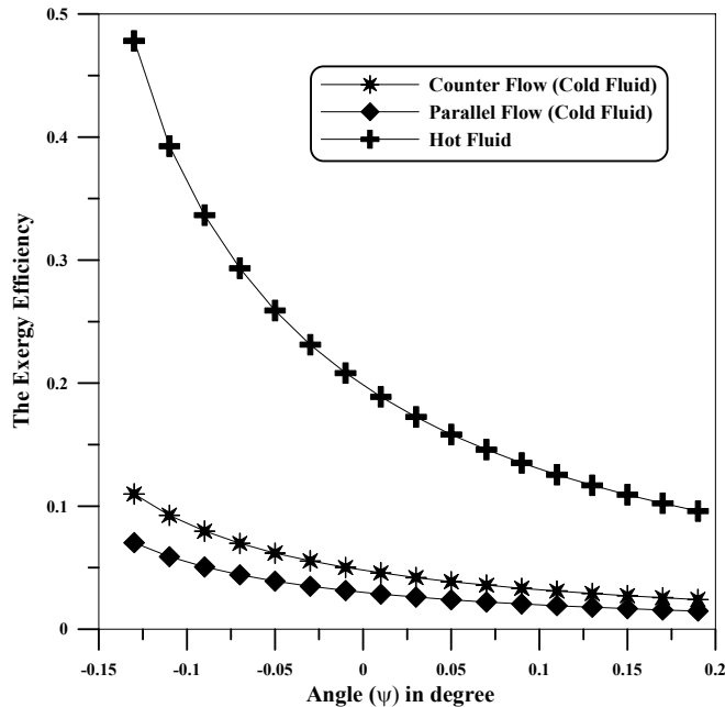
Figure (11), History of fluid exergy effectiveness (hot and cold) for different values of ( \psi )
